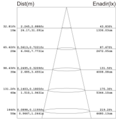
100W-Lux Distance Cure
