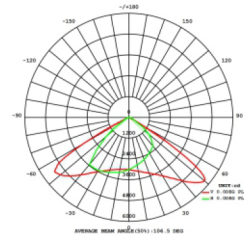
100W-Light Distribution Curve
