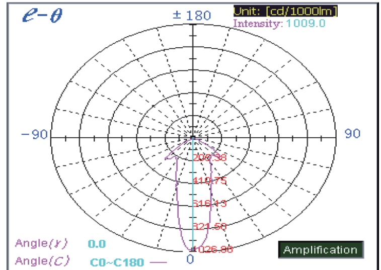
Light Distribution Curve
