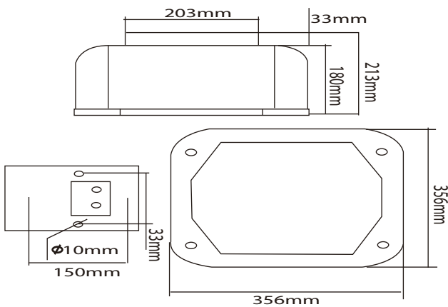
Product Dimensions
